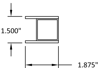
10 HEAD AND HINGE STILE STEEL
