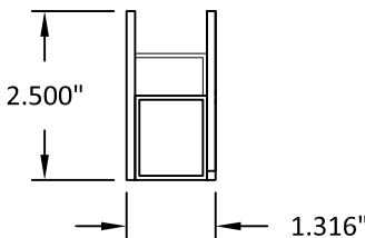
9 LOCK STILE STEEL
