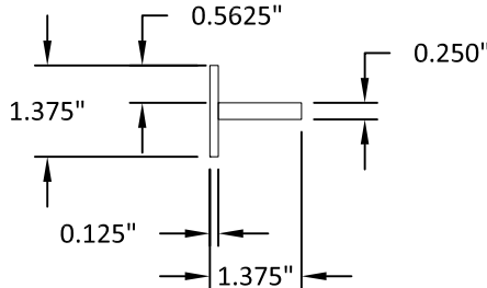
12 TDL STEEL
