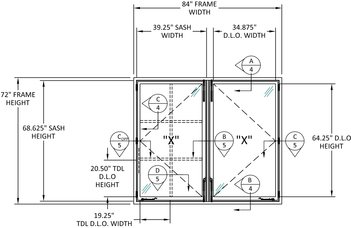
ELEVATION DOUBLE CASEMENT
