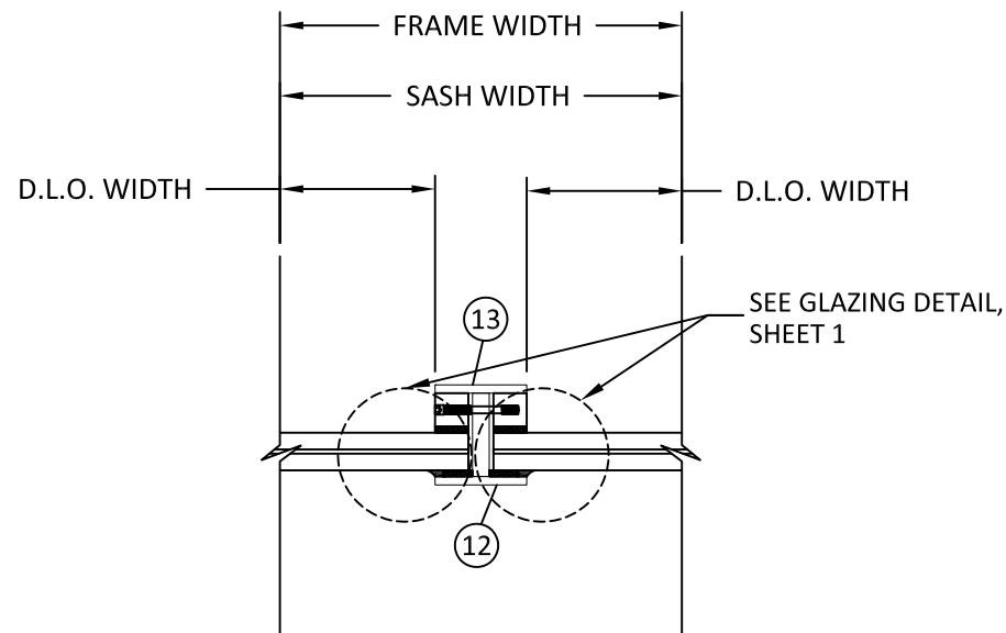
B HORIZONTAL SECTION 5 MULLION
