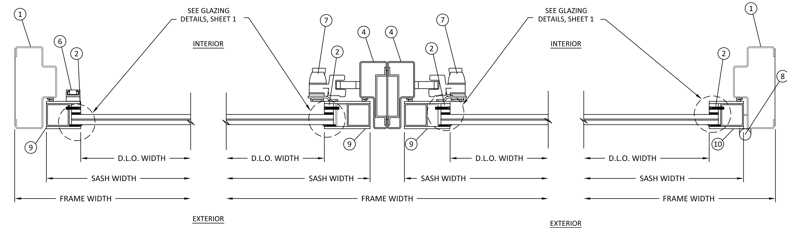
A HORIZONTAL SECTION 5 LOCK JAMB
