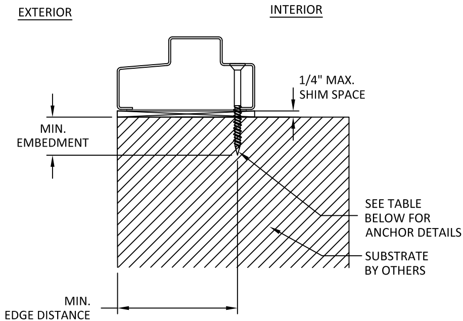
B 6 VERTICAL SECTION SILL - THROUGH FRAME
