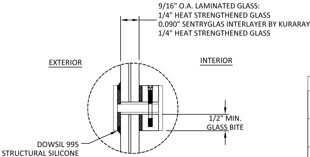
GLAZING DETAIL 2
