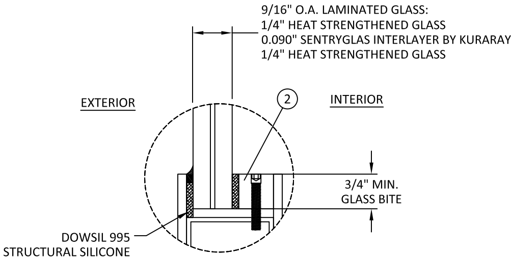
GLAZING DETAIL 1
