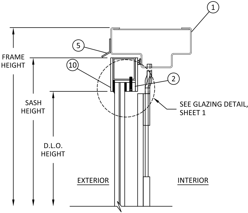
A 4 VERTICAL SECTION HEAD
